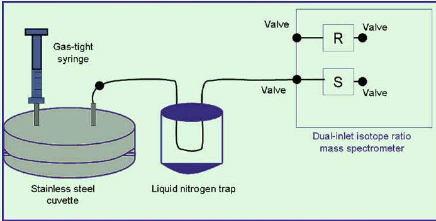
FIGURE 1. Diagram of an on-line oxygen-isotope fractionation system, with a gas-tight syringe, a stainless steel cuvette, a liquid nitrogen trap to remove \text{CO}_2
