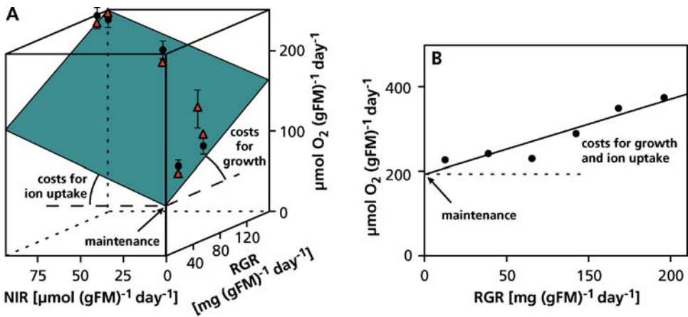
FIGURE 26. (A) Rate of O_2 consumption per unit fresh mass (FM) in roots as related to both the relative growth rate (RGR) of the roots and their net rate of anion uptake (NIR). (B) Rate of O_2 consumption per unit fresh mass in roots as related to the relative growth rate of the roots. The plane in (A) and line in (B) give the predicted mean rate of O_2 consumption. The intercept of the plane in (A) and the line in (B) with the y-axis
