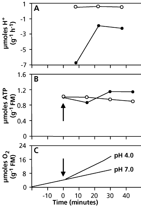
FIGURE 18. Effect of the pH in the rhizosphere on (A) net \text{H}^+ release, (B) ATP concentration, and (C) respiration of Zea mays (maize) roots. Seedlings were grown at pH 7.0, and either kept at pH 7.0 (open symbols) or exposed to a pH of 4.0 (filled symbols) at the time indicated by the arrow. Note that the slopes in A and C give the rate of \text{H}^+ release and respiration (after Yan et al. 1992). Copyright American Society of Plant Biologists.
