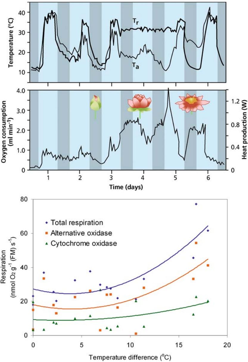
FIGURE 10. (Top) Temperature of the receptacle ( T_r ) and ambient air ( T_a ) and (Middle) rates of O_2 consumption throughout the thermogenic phase in Nelumbo nucifera (sacred lotus). O_2 consumption is converted to heat production assuming 21.1 \text{ J ml}^{-1} of O_2 . Shaded areas indicate the night period (Seymour & Schultze-Motel 1996). Reprinted with permission from Nature copyright 1996 MacMillan Magazines Ltd. (Bottom) Total respiratory flux and fluxes through the alternative and cytochrome pathways, in lotus receptacle tissues as a function of the difference between receptacle temperature and temperature of an adjacent nonheating receptacle. Partitioning of electron transport between the two respiratory pathways was determined on the basis of ^{18}O -isotope fractionation of intact tissues, as described in Box 2B.1 (modified after Watling et al. 2006). Copyright American Society of Plant Biologists.
