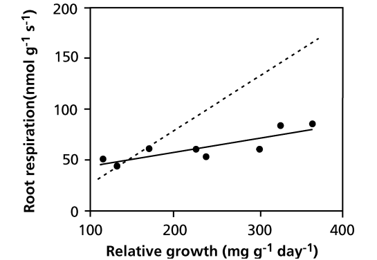
FIGURE 27. The rate of root respiration of fast-growing and slow-growing herbaceous C 3 species. The broken line gives the calculated respiration rate, assuming that specific costs for growth, maintenance, and ion uptake are the same as those given in Table 11 and identical for all investigated species (Poorter et al. 1991). Copyright Physiologia Plantarum.
