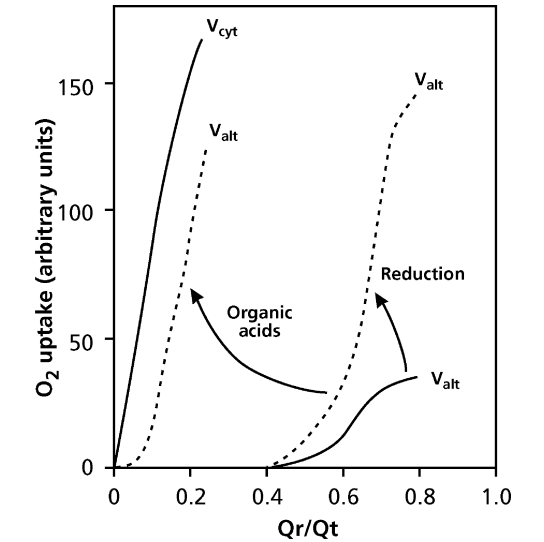
FIGURE 8. Dependence of the activity of the cytochrome path and of the alternative path on the fraction of ubiquinone that is in its reduced state ( Q_r/Q_t ). When the alternative oxidase is in its “reduced” (higher-activity) configuration, it has a greater capacity to accept electrons. In its reduced state, the alternative oxidase can be affected by \alpha -keto acids, which enhance its activity at low levels of Q_r . [Based on Dry et al. (1989), Umbach et al. (1994), Day et al. (1995), and Hoefnagel et al. (1997)].
