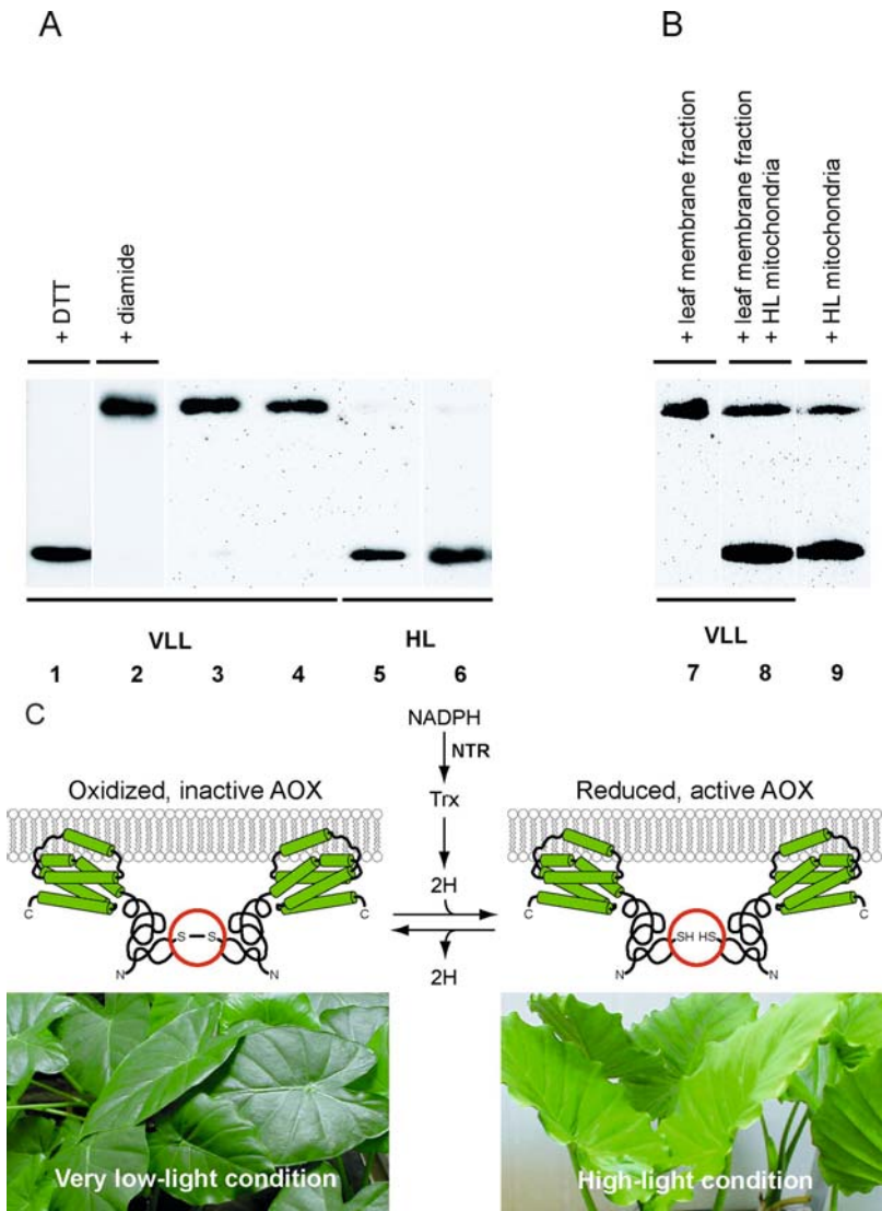
FIGURE 16. (A) Immunoblots of the alternative oxidase (AOX) in extracted membrane fractions isolated from Alocasia odora (Asian taro) leaves. Extractions were made very rapidly, so as to maintain the activation state of AOX and determine its in vivo state. Lane 1, a sample of leaves of plants grown at very low light intensities (VLL) treated in the presence of 50 mM DTT (dithiothreitol, which renders AOX in its reduced and active state, irrespective of its state in vivo ). Lane 2, a sample of VLL leaves treated in the presence of 5 mM diamide (which oxidizes and inactivates the AOX dimer, irrespective of its state in vivo ). Lanes 3 and 4, samples consisted of only VLL leaf membrane fractions; the immunoblots show that AOX was in its oxidized, inactive state in leaves of plants grown at very low light intensity. Lanes 5 and 6, samples consisted of only high-light grown (HL) leaf membrane fractions; these immunoblots show that AOX was in its reduced, active state in leaves of plants grown at high light intensity. (B)
